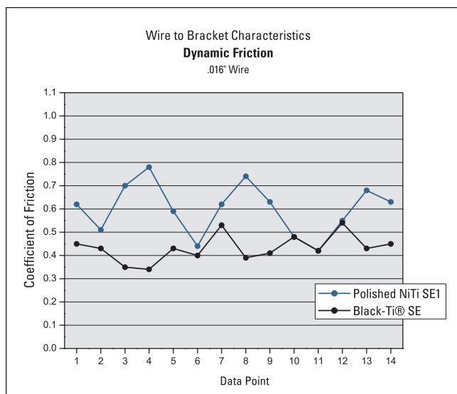
These graphs compare the friction characteristics as wire slides through a bracket.
